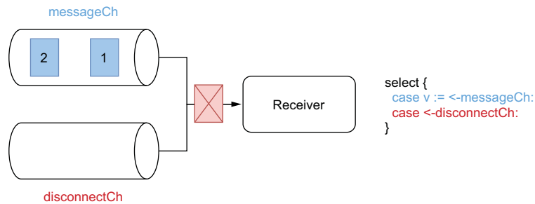
Figure 9.3 Receiving the disconnection
