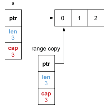
Figure 4.1 s is copied to a temporary variable used by range .
