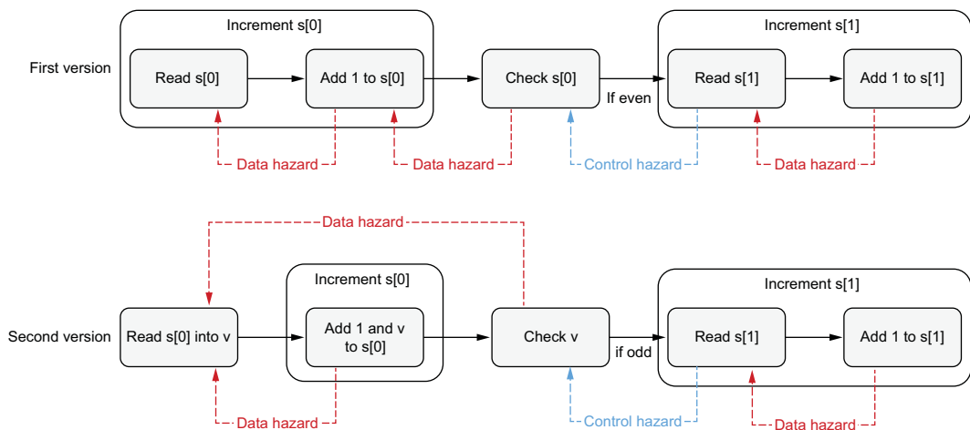
Figure 12.19 One significant difference: the data hazard for the v check step
