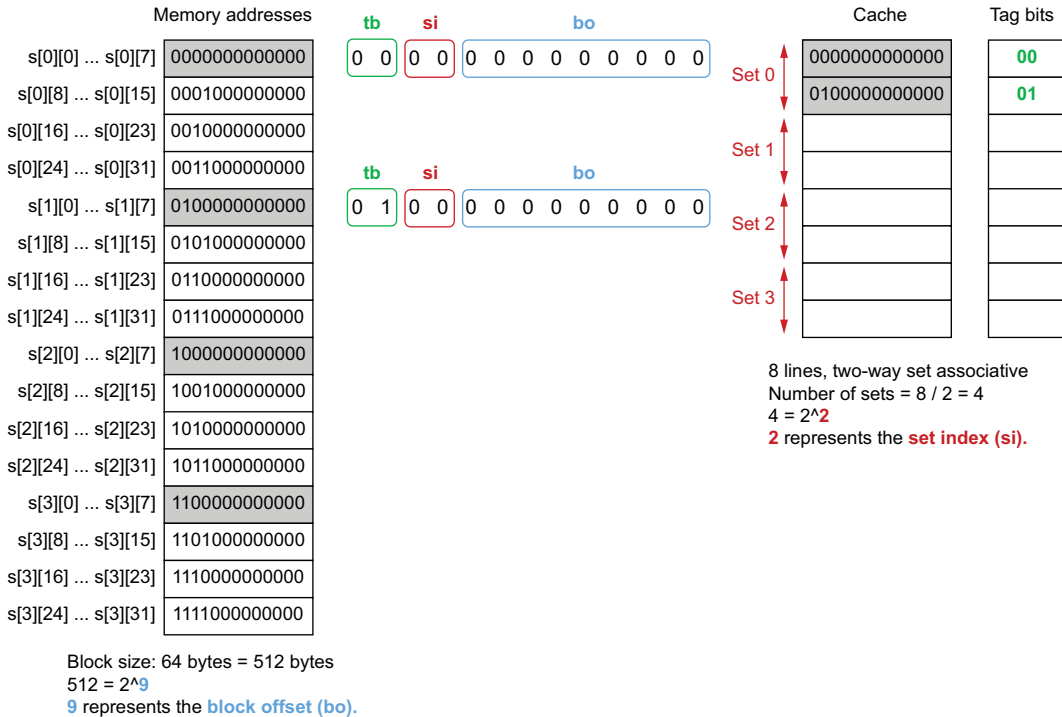
Figure 12.9 Memory address 0100000000000 is copied into set 0.
