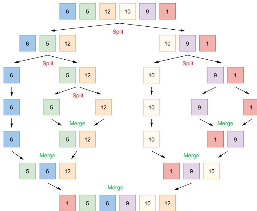
Figure 8.7 Applying the merge sort algorithm repeatedly breaks each list into two sublists. Then the algorithm uses a merge operation such that the resulting list is sorted.
