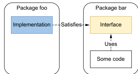
The interface lives on the consumer side.
