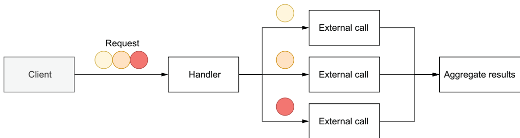
Figure 9.13 Each circle results in a parallel call.
