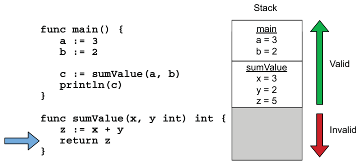
Figure 12.27 Calling sumValue creates a new stack frame.
