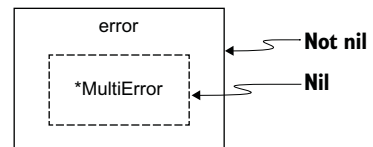
Figure 6.1 The error wrapper isn't nil .
