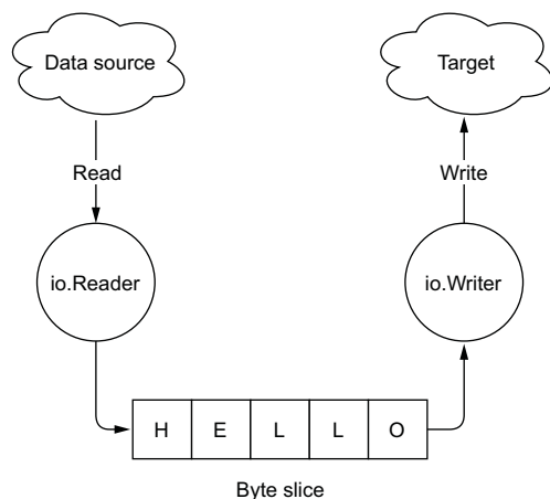
Figure 2.3 io.Reader reads from a data source and fills a byte slice, whereas io.Writer writes to a target from a byte slice.
