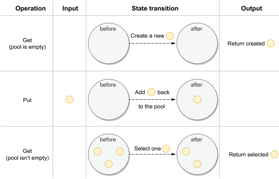
Figure 12.33 Get either creates a new object or returns one from the pool. Put returns the object to the pool.
