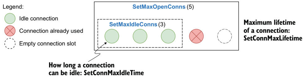
Figure 10.1 A connection pool with five connections
