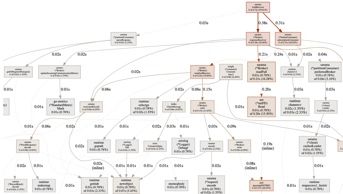
Figure 12.34 The call graph of an application during 30 seconds
