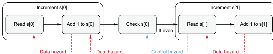
Figure 12.17 Hazard types between the instructions
