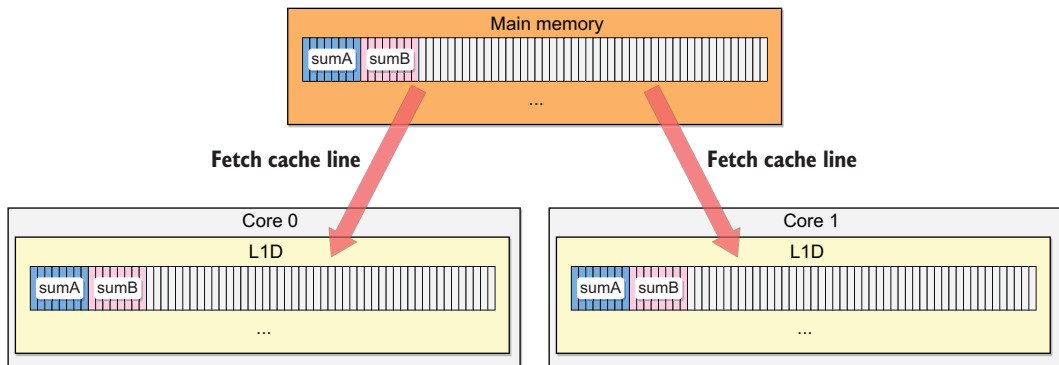
Figure 12.12 Each block is copied to a cache line on both core 0 and core 1.
