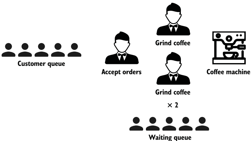
Figure 8.4 Hiring another waiter to grind coffee beans
