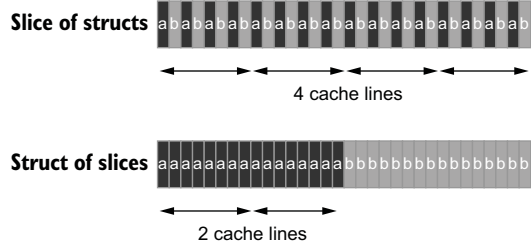
Figure 12.4 A struct of slices is more compact and therefore requires fewer cache lines to iterate over.
