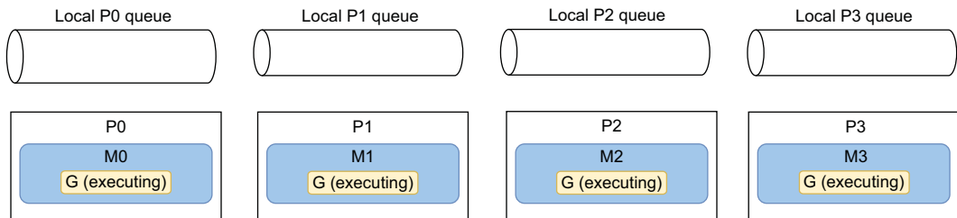
Figure 8.14 At most four goroutines are now running.
