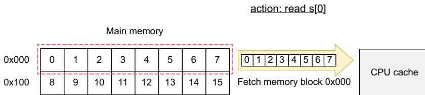
Figure 12.2 Accessing s[0] makes the CPU copy the 0x000 memory block.
