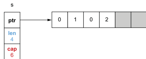
Figure 3.4 Appending an element to s
