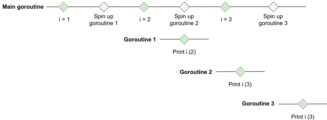
Figure 9.1 The goroutines access an i variable that isn't fixed but varies over time.
