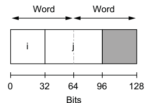
Figure 12.21 j allocated on two words
