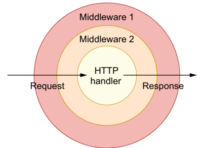
Figure 8.15 Before reaching the handler, a request goes through the configured middleware.
