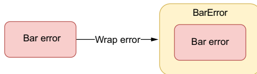
Figure 7.5 Wrapping the error inside BarError
