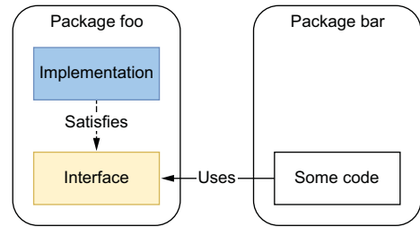
The interface lives on the producer side.
