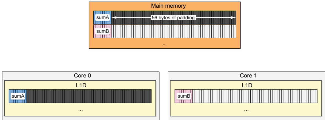
Figure 12.14 sumA and sumB are part of different memory blocks.
