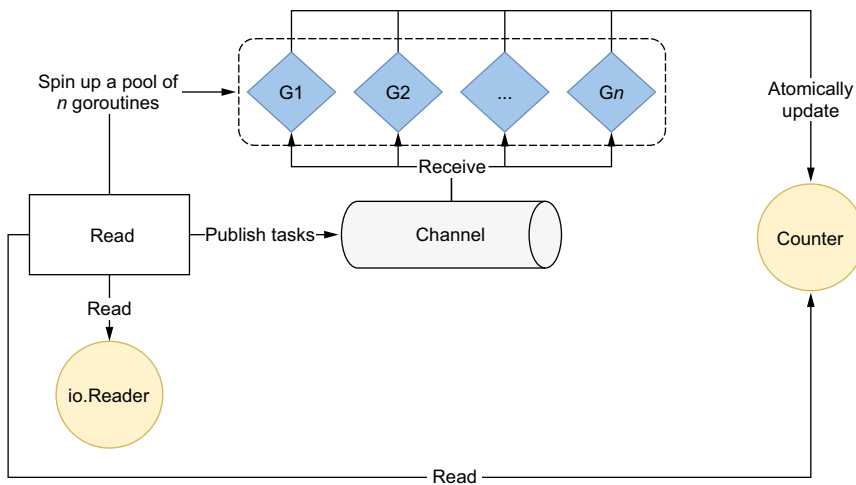
Figure 8.11 Each goroutine from the fixed pool receives from a shared channel.
