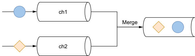
Figure 9.7 Merging two channels into one
