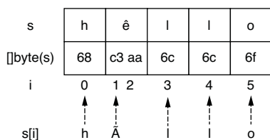
Figure 5.1 Printing s[i] prints the UTF-8 representation of each byte at index i .
