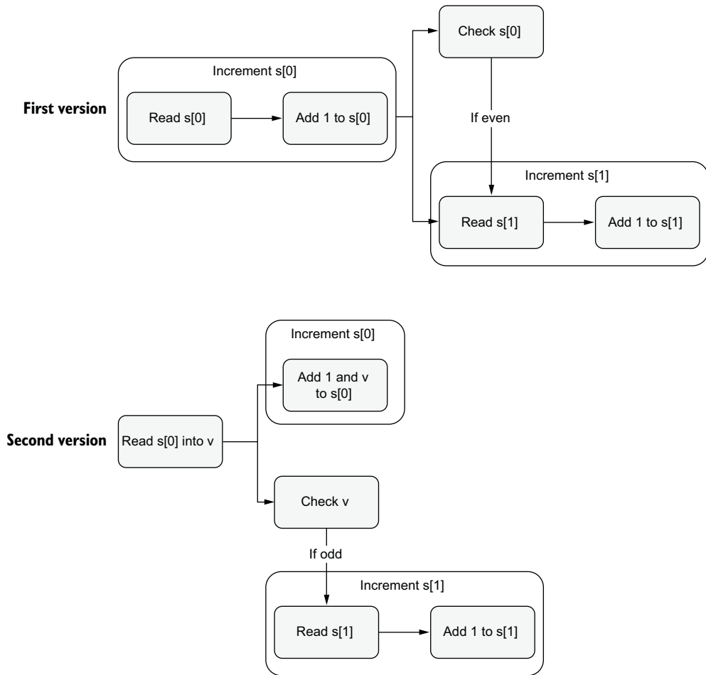
Figure 12.20 In the second version, both increment steps can be executed in parallel.
