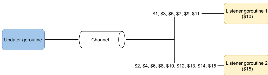
Figure 9.12 The first goroutine receives the $1 message, then the second goroutine receives the $2 message, then the first goroutine receives the $3 message, and so forth.
