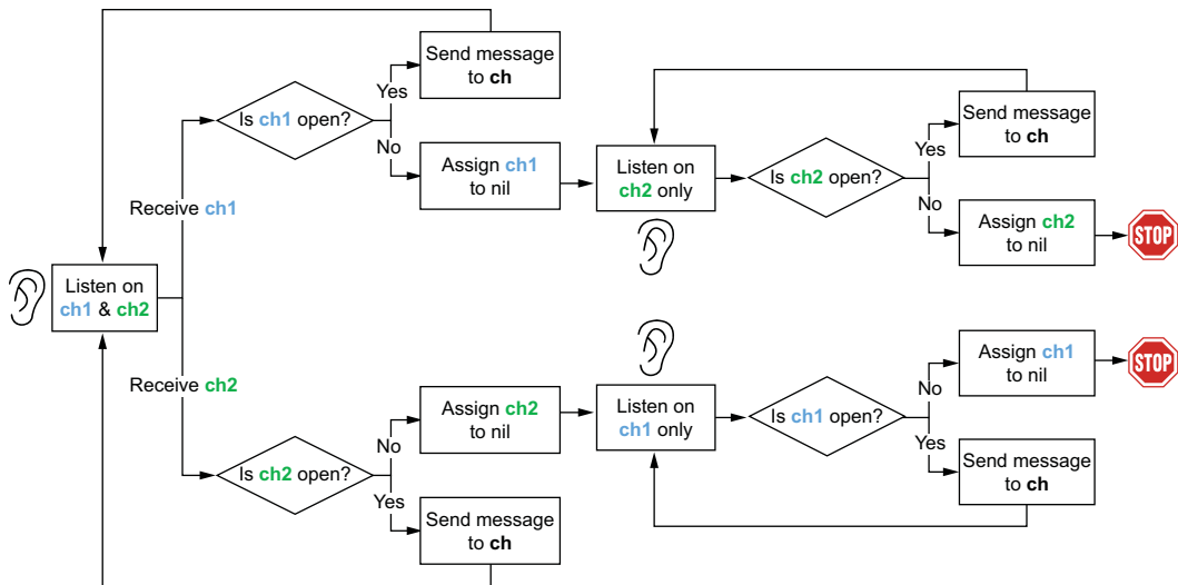
Figure 9.9 Receiving from both channels. If one is closed, we assign it to nil so we only receive from one channel.
