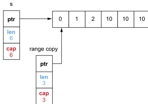
Figure 4.2 The temporary variable remains a three-length slice; hence, the iteration completes.
