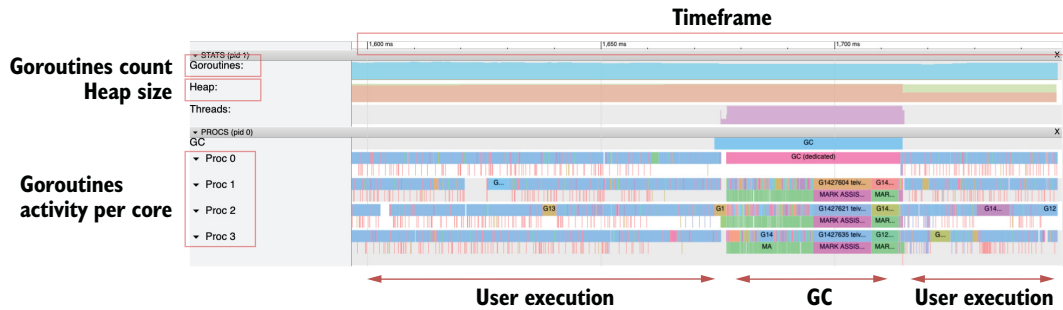
Figure 12.39 Showing goroutine activity and runtime events such as a GC phase
