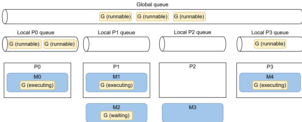
Figure 8.6 An example of the current state of a Go application executed on a four-core machine. Goroutines that aren't in an executing state are either runnable (pending being executed) or waiting (pending a blocking operation).
