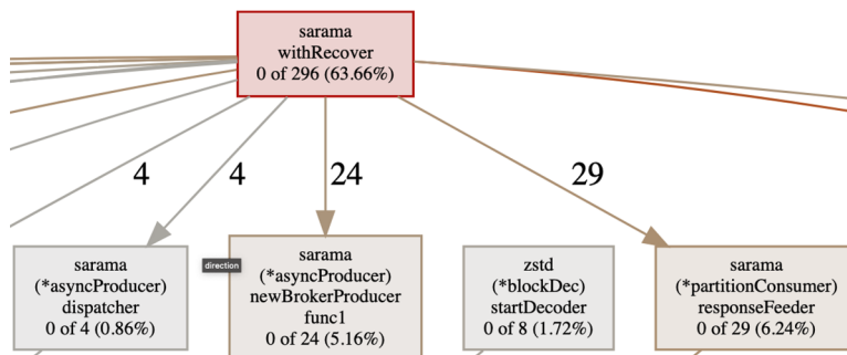
Figure 12.38 Goroutine graph
