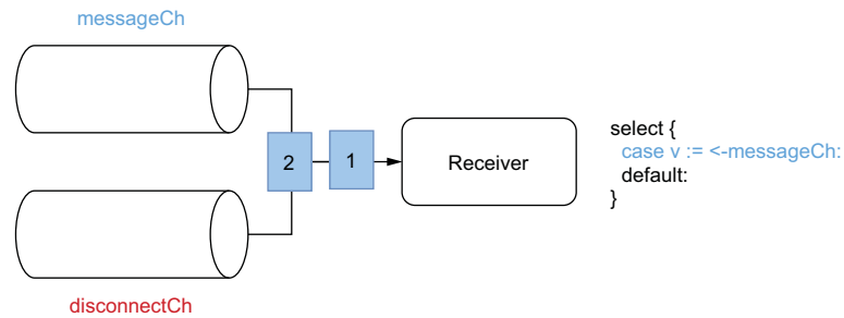
Figure 9.5 Receiving the remaining messages
