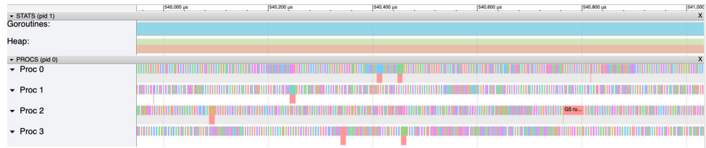
Figure 12.40 Too many small bars mean poorly parallelized execution.
