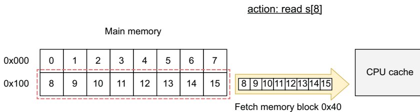
Figure 12.3 Accessing s[8] makes the CPU copy the 0x100 memory block.
