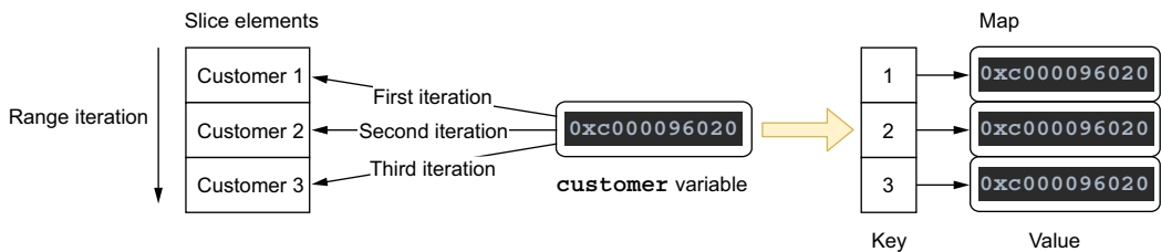
Figure 4.4 The customer variable has a constant address, so we store in the map the same pointer.
