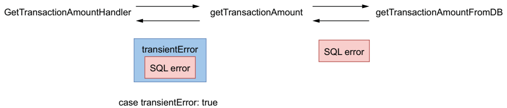
Figure 7.8 Because getTransactionAmount returned a transientError if the DB failed, the case was true.
