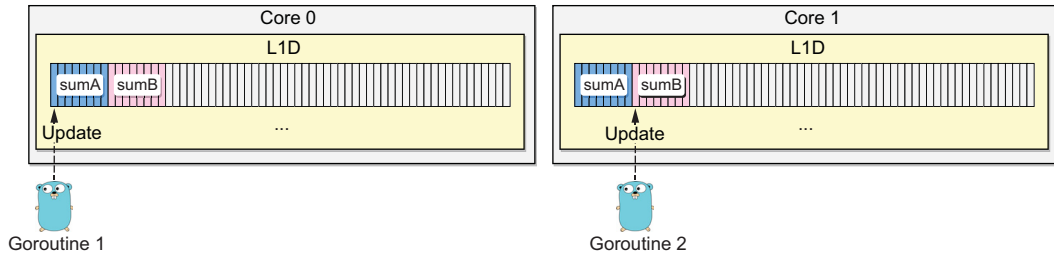
Figure 12.13 Each goroutine updates its own variable.
