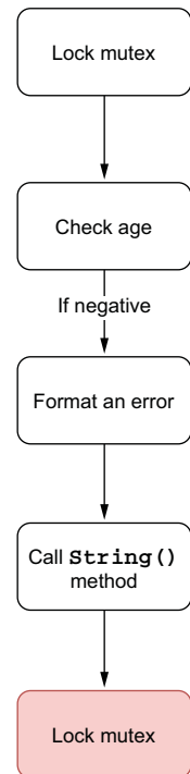
Figure 9.10 UpdateAge execution if age is negative
