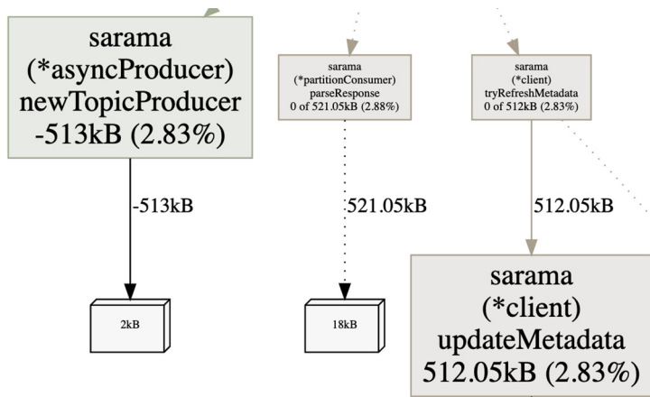
Figure 12.37 The differences between the two heap profiles
