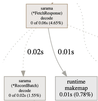
Figure 12.35 Example call graph
