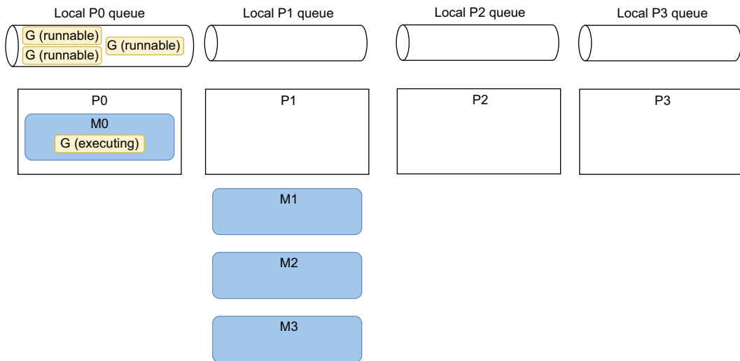
Figure 8.12 At most one goroutine is running.
