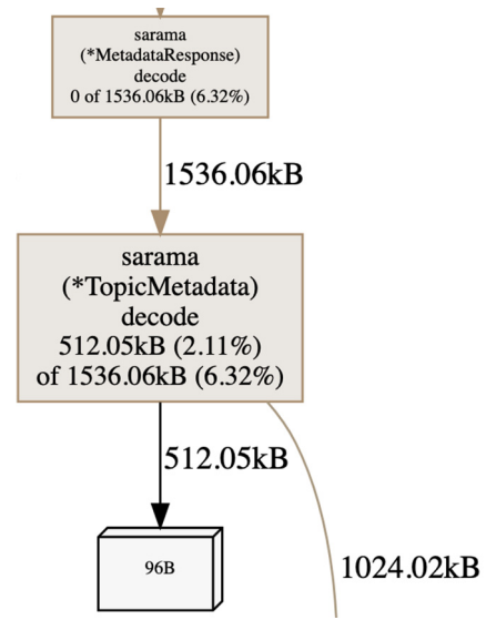
Figure 12.36 A heap graph
