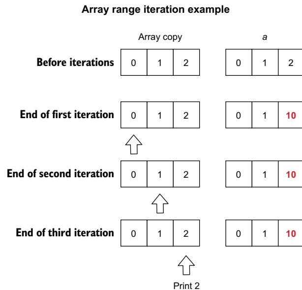
Figure 4.3 range iterates over the array copy (left) while the loop modifies a (right).
