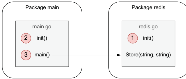
Figure 2.2 The init function of the redis package is executed first, then the init function of main , and finally the main function.
