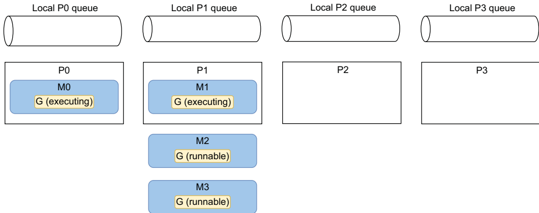
Figure 8.13 At most two goroutines are running.
