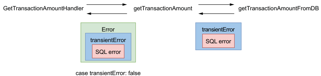
Figure 7.9 Now getTransactionAmount returns a wrapped error. Hence, case transientError is false.
