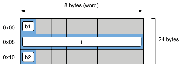
Figure 12.23 The struct occupies 24 bytes total.
