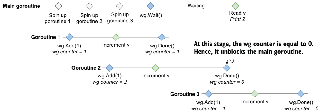
Figure 9.11 The last goroutine calls wg.Add(1) after the main goroutine is already unblocked.
