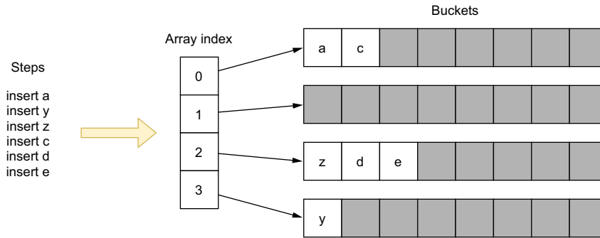
Figure 4.5 A map with four buckets
