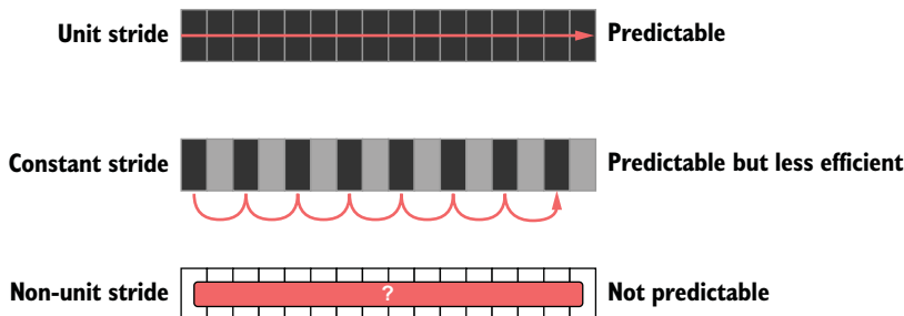
Figure 12.6 The three types of strides
