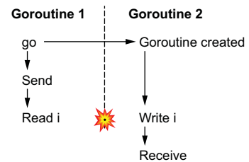
Figure 8.9 If the channel is buffered, it leads to a data race.
