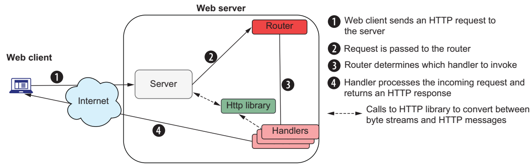
Figure 2.8 Web server message flow
