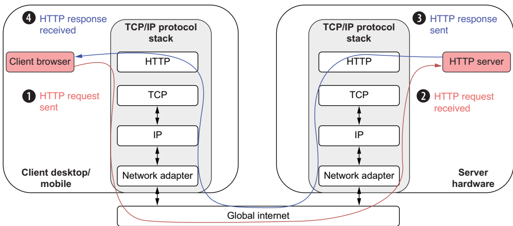
Figure 2.4 HTTP communications with a protocol stack
