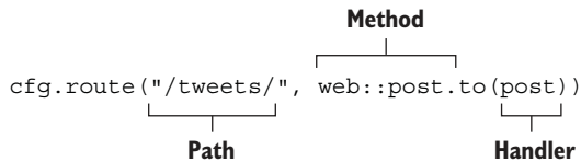
Figure 3.2 Structure of an Actix route
